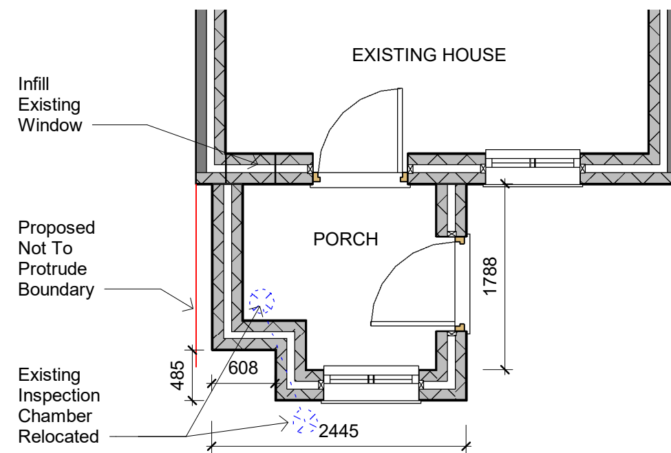
PORCH FLOOR PLAN
