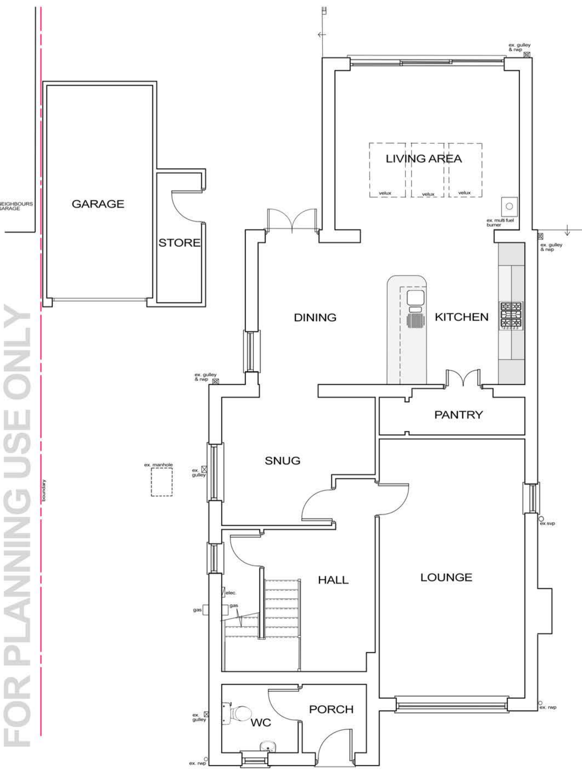
EXISTING GROUND FLOOR 1:50
