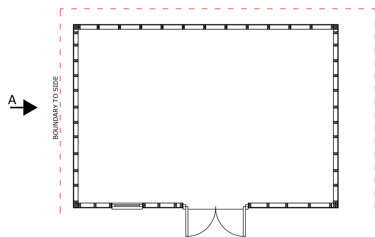
GROUND FLOOR PLAN AS PROPOSED (BUILT) 1:50
