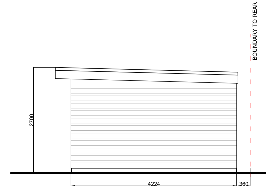
ELEVATION ON B
