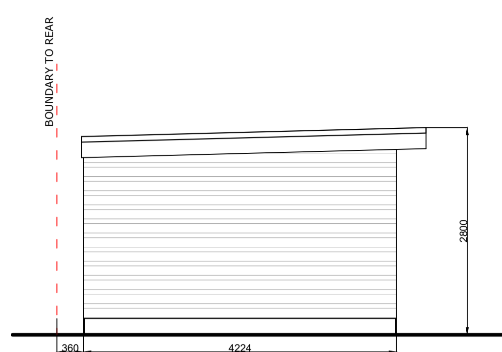
ELEVATION ON A
