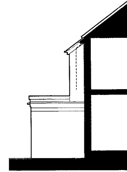
SIDE ELEVATION AT REAR
