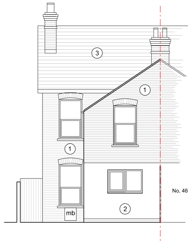
Existing Rear / South-East Elevation
