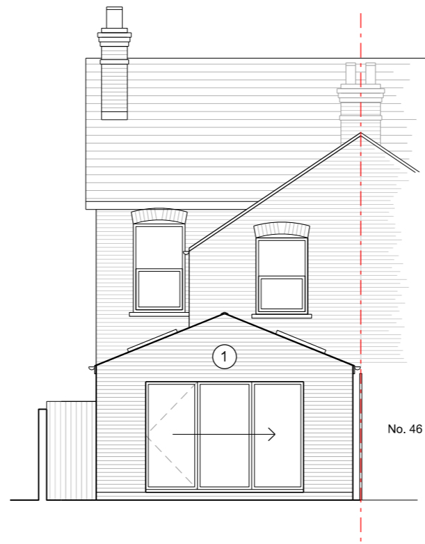
Proposed Rear / South-East Elevation
