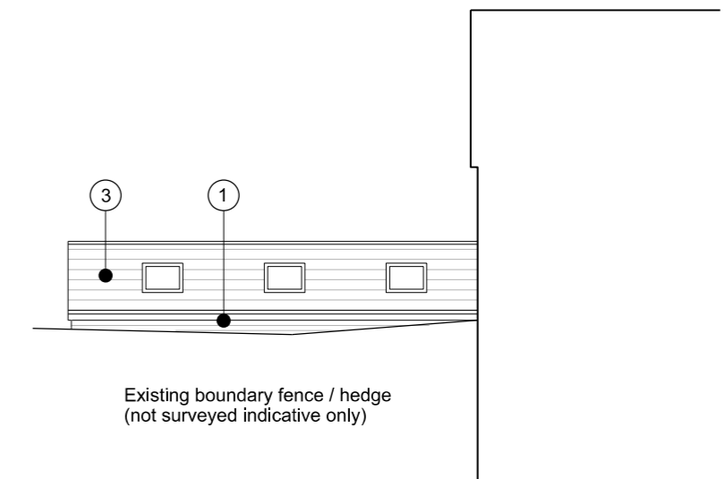
Proposed Side / North-East Sectional Elevation Facing No. 46
