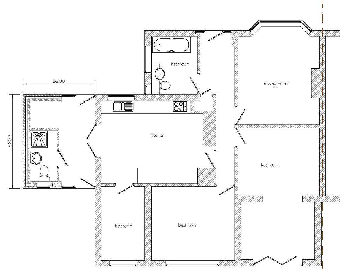
Proposed Ground Floor Layout
