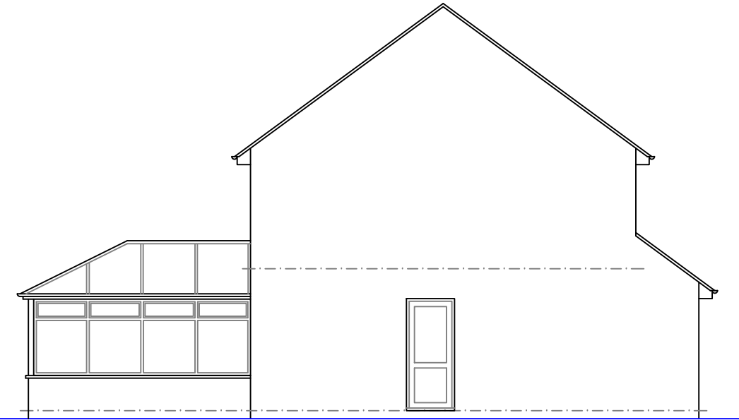
SIDE ELEVATION
