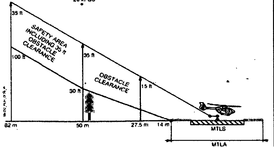
Fig. C2 Landing flight path obstacle clearance
